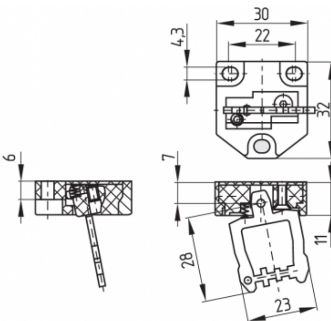
Flexible actuator B6R
