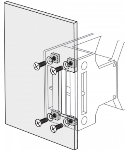
Front mounting
