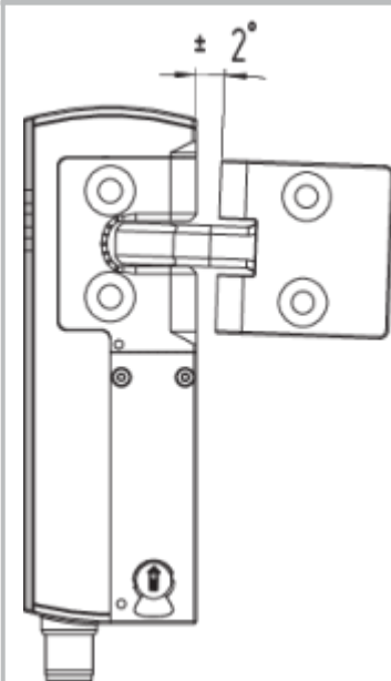
Tilt angle
