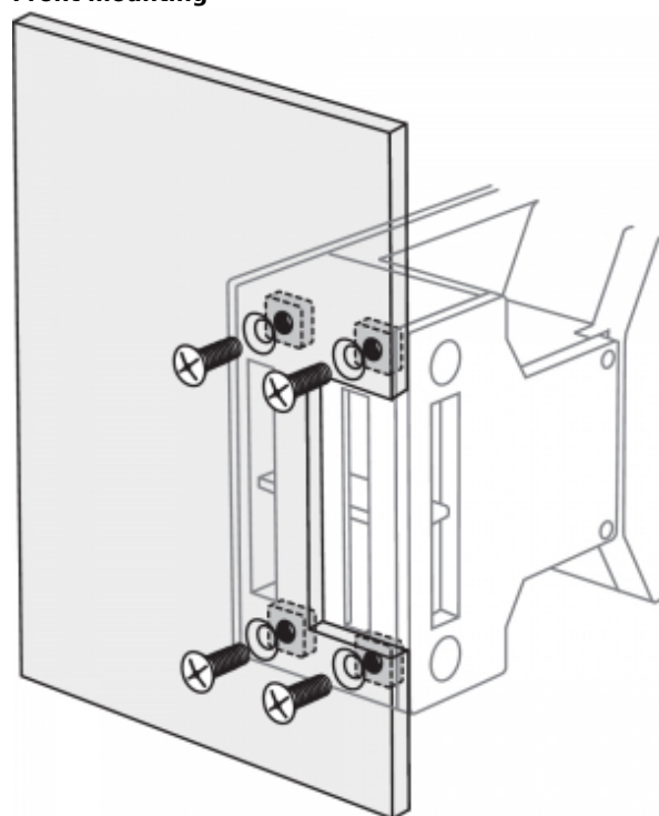
Front mounting
