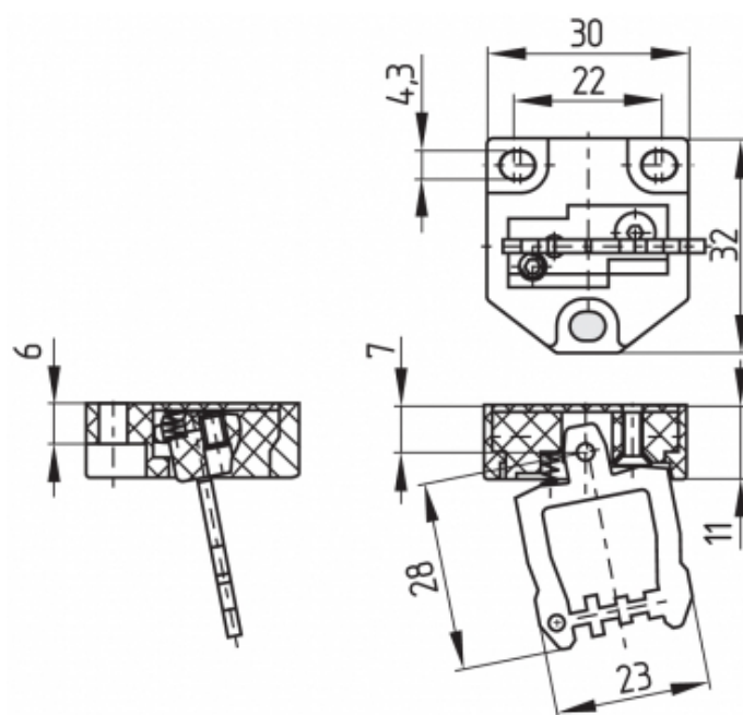
Flexible actuator B6R
