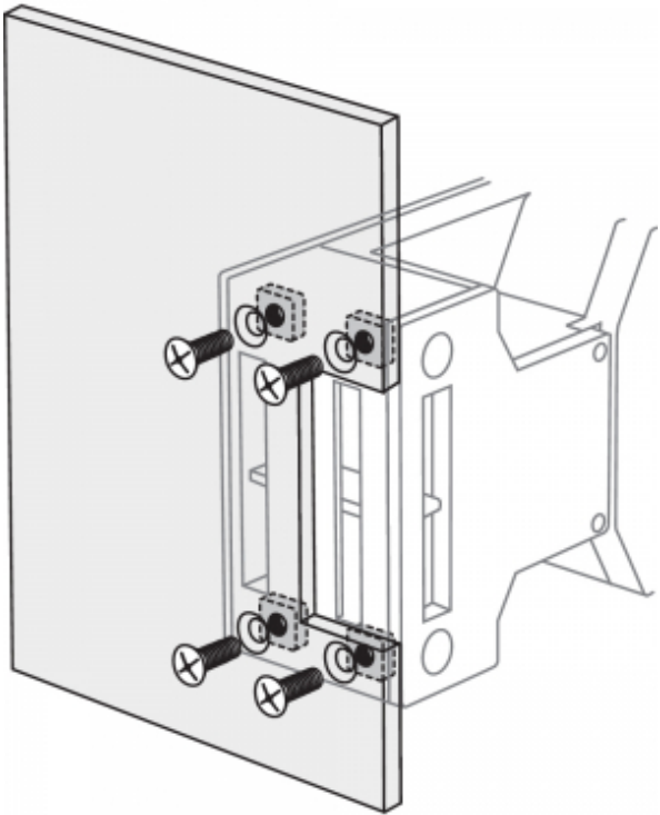
Front mounting
