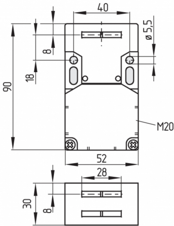
Front mounting
