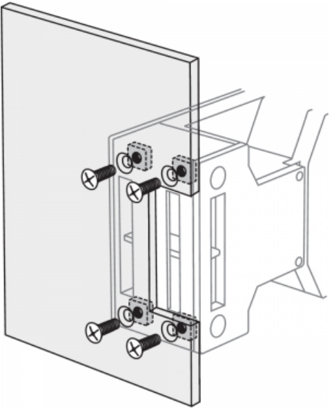
Front mounting
