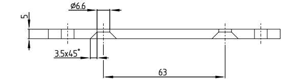
Lockout tag SZ400 (available as accessory) For detailed information and assembly instructions, see operating instructions SZ400.
