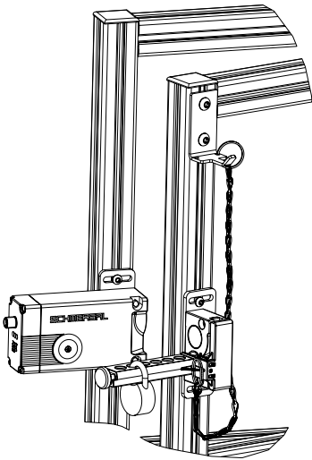
Bowden cable release ACC-AZM400-BOW-M-M (available as accessory) Observe the additional notes in the operating instructions of the Bowden cable release.
