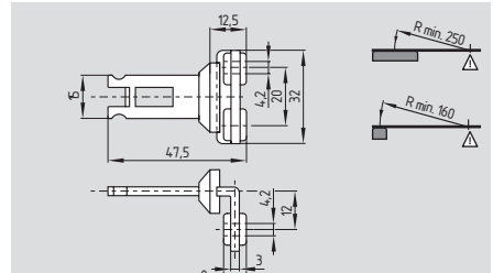
Shortened angled actuator TZ/CWK
