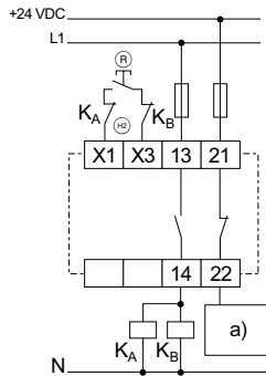
Fig. 18 a) Control Ⓡ = Reset button Ⓢ = Feedback circuit
