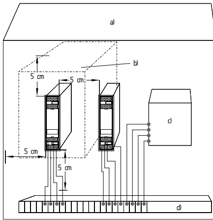
Fig. 1 a) IP54 control box suitable for installation in Zone 2 in accordance with EN IEC 60079-7 (ABNT NBR IEC 60079-7), EN IEC 60079-15 (ABNT NBR IEC 60079-15) b) Air around the safety-monitoring module approx. 2,400 cm 3 (8.25 × 16 × 18.1 cm) c) Protection (suitable for Zone 2) d) Clips (suitable for Zone 2)
