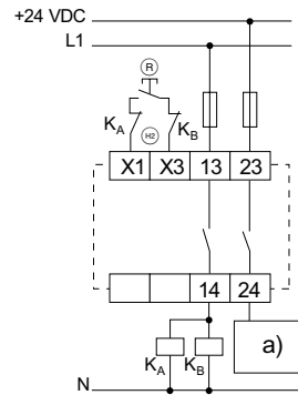
Fig. 18 a) Control Ⓡ = Reset button Ⓢ = Feedback circuit
