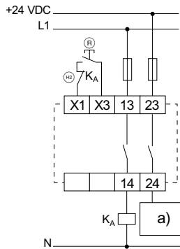
Fig. 17 a) Control Ⓡ = Reset button Ⓢ = Feedback circuit
