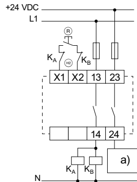
Fig. 17 a) Control Ⓡ = Reset button Ⓢ = Feedback circuit
