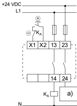
Fig. 16 a) Control Ⓡ = Reset button Ⓢ = Feedback circuit
