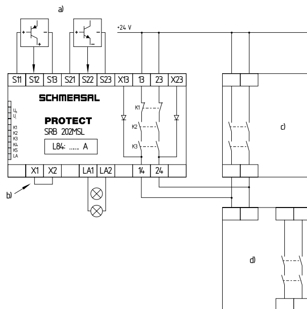
Fig. 7 a) Semi-conductor muting sensors, b) Bridge, c) AOPD (relay outputs), d) Schmersal-SRB
