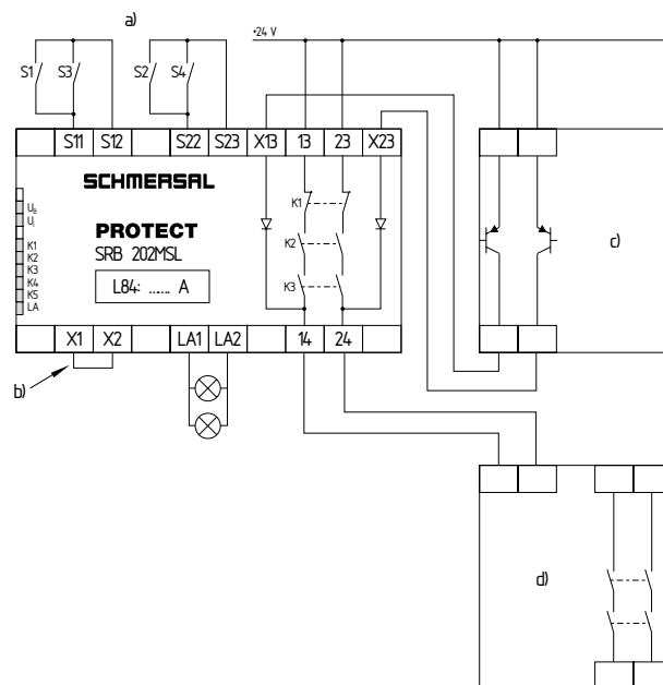
Fig. 6 a) Muting sensors, b) Bridge, c) AOPD (semi-conductor outputs), d) Schmersal-SRB
