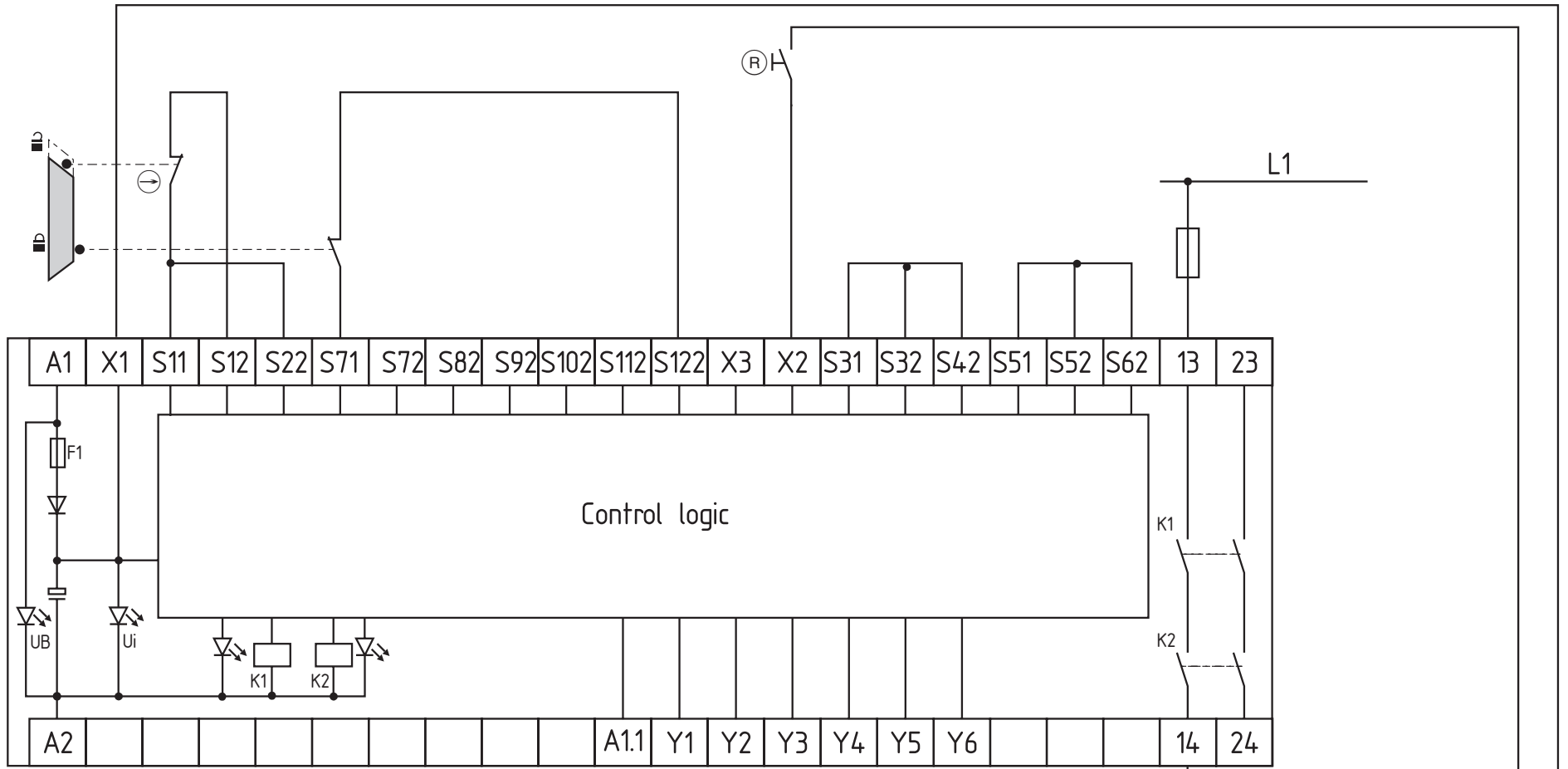
SRB 206SQ
