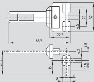
Angled actuator EX-BOW
