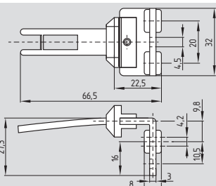
Angled radius actuator EX-BOWR
