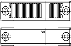
Actuator RST 36-1 / RST 36-1-R
