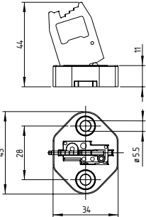
Installation position with actuator inserted (all measurements ± 0.3 mm)
