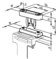
Actuator B1-2177 with centering guide
