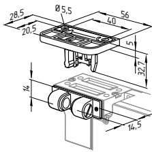
Actuator B1-2053 with ball latch
